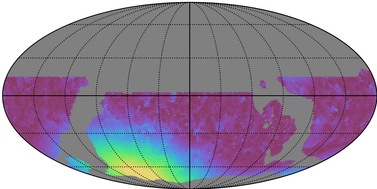
ddf_loaded_fl2_v3.4_10yrs WFD r band: Min moonDistance
