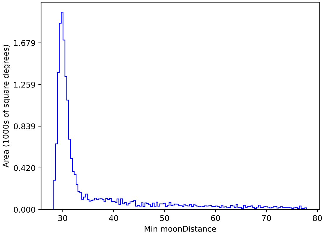
ddf_loaded_fl2_v3.4_10yrs WFD i band: Min moonDistance
