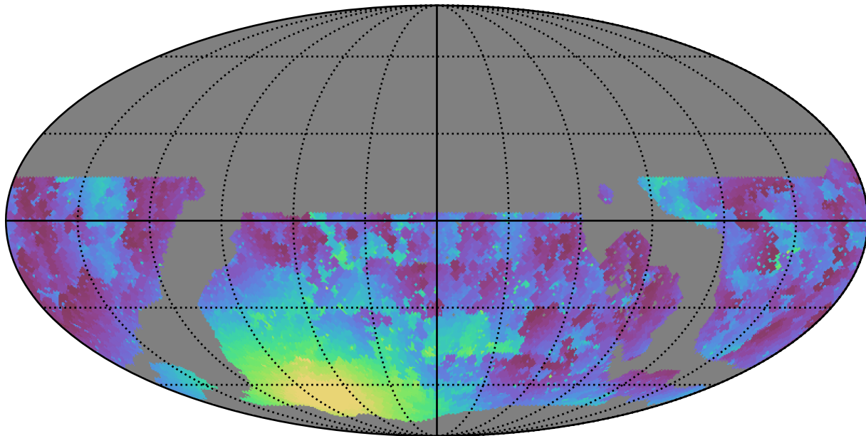
ddf_loaded_fl2_v3.4_10yrs WFD g band: Min moonDistance
