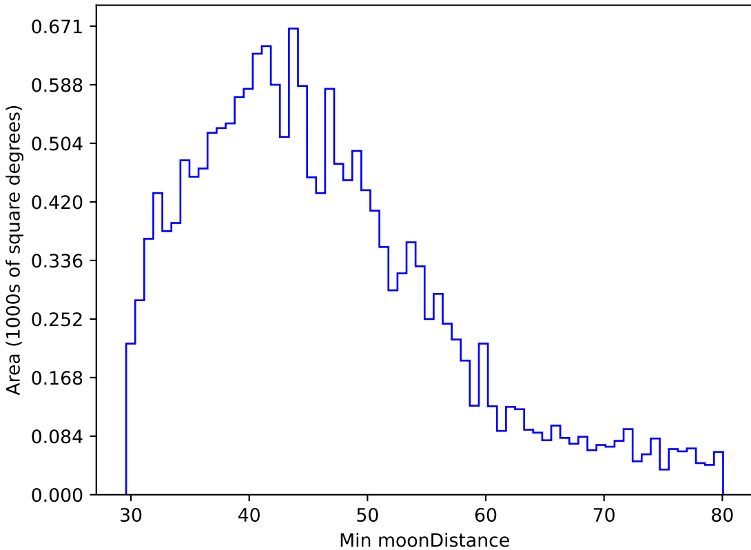
ddf_loaded_fl2_v3.4_10yrs WFD g band: Min moonDistance
