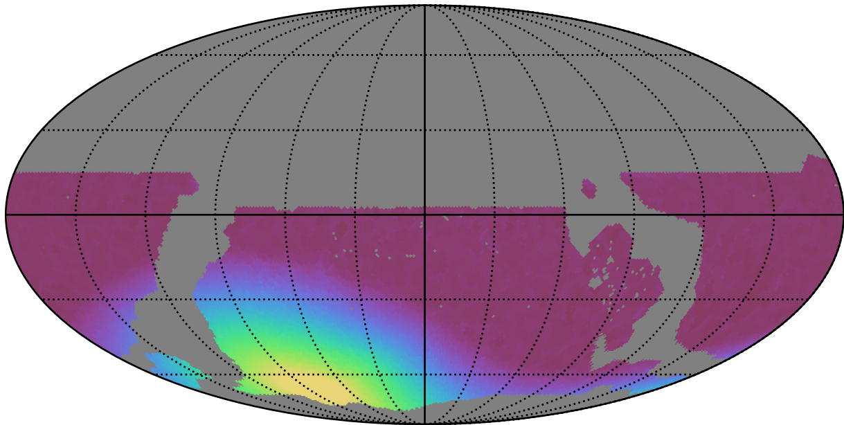
ddf_loaded_fl2_v3.4_10yrs WFD all bands: Min moonDistance
