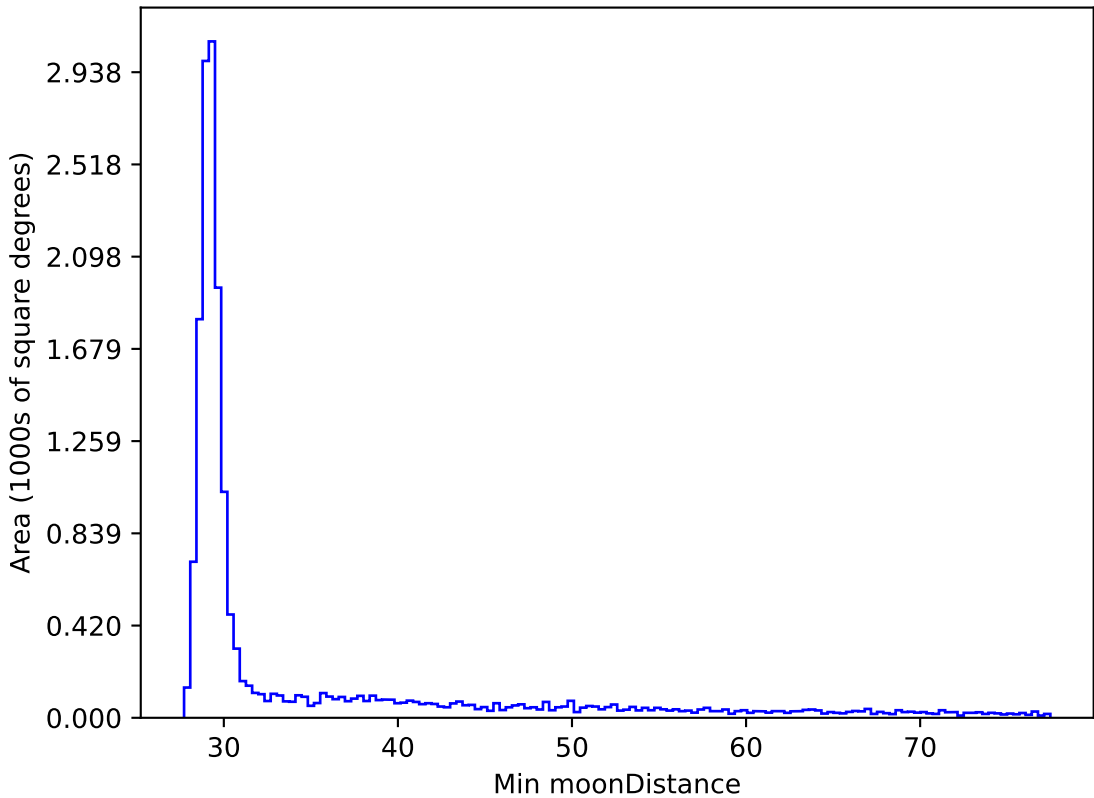
ddf_loaded_fl2_v3.4_10yrs WFD all bands: Min moonDistance
