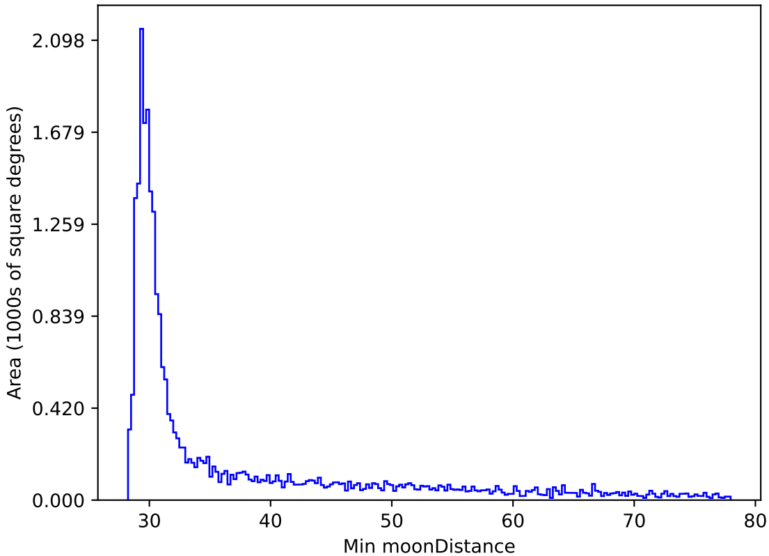
ddf_loaded_fl2_v3.4_10yrs All sky z band: Min moonDistance
