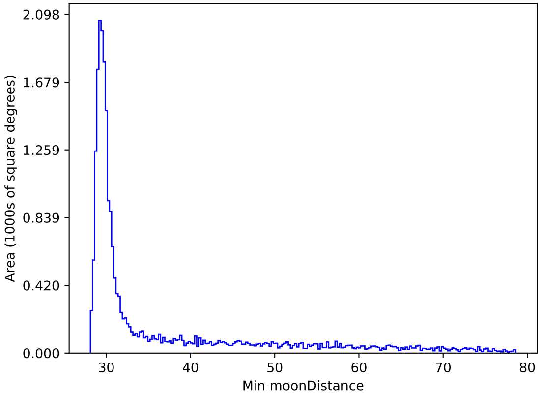
ddf_loaded_fl2_v3.4_10yrs All sky y band: Min moonDistance
