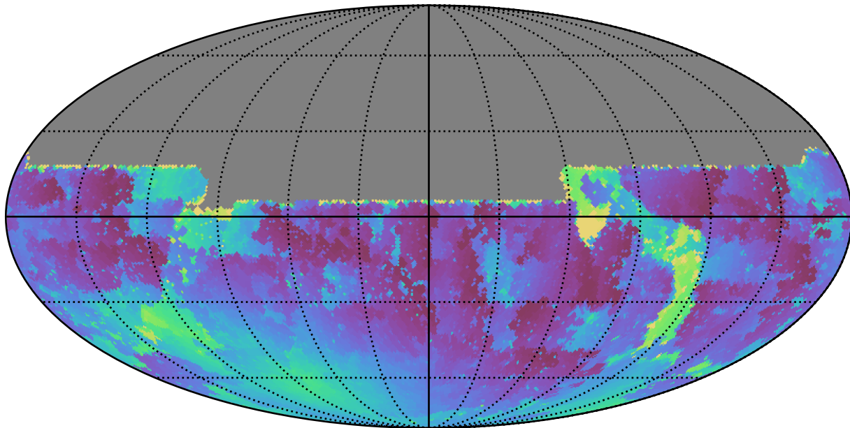
ddf_loaded_fl2_v3.4_10yrs All sky u band: Min moonDistance
