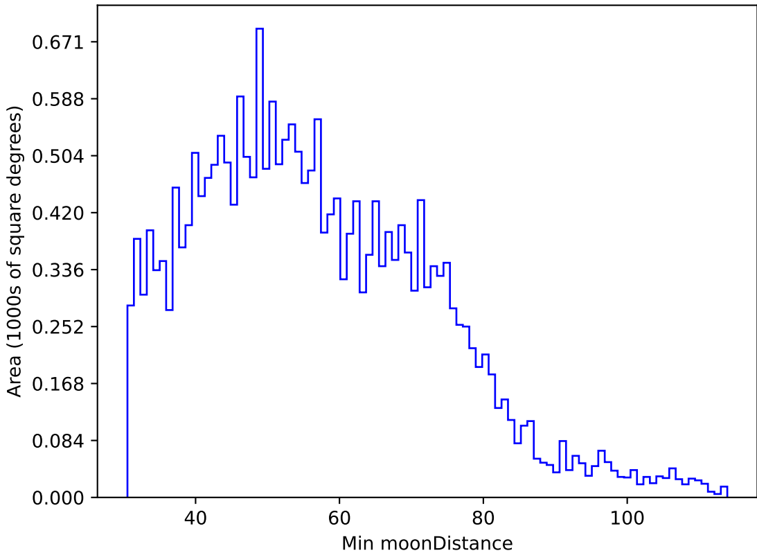
ddf_loaded_fl2_v3.4_10yrs All sky u band: Min moonDistance
