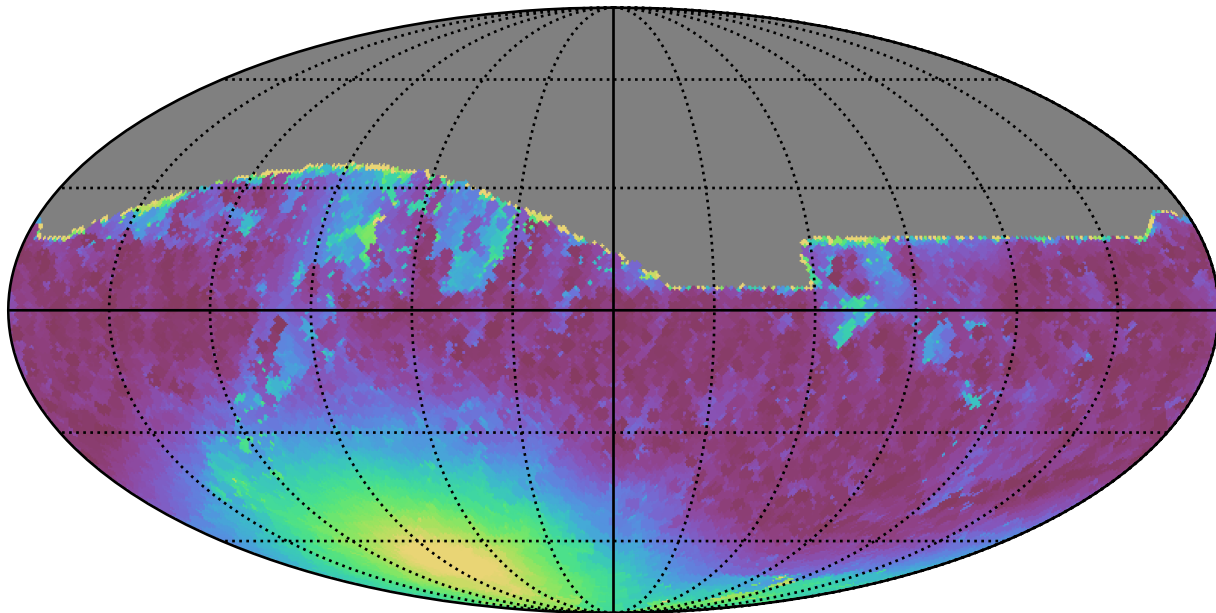
ddf_loaded_fl2_v3.4_10yrs All sky r band: Min moonDistance
