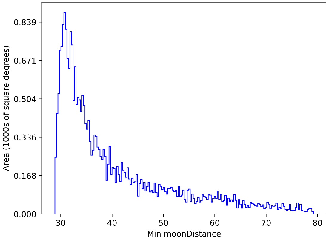
ddf_loaded_fl2_v3.4_10yrs All sky r band: Min moonDistance
