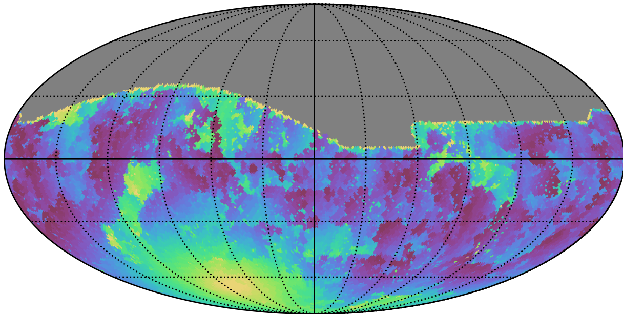
ddf_loaded_fl2_v3.4_10yrs All sky g band: Min moonDistance
