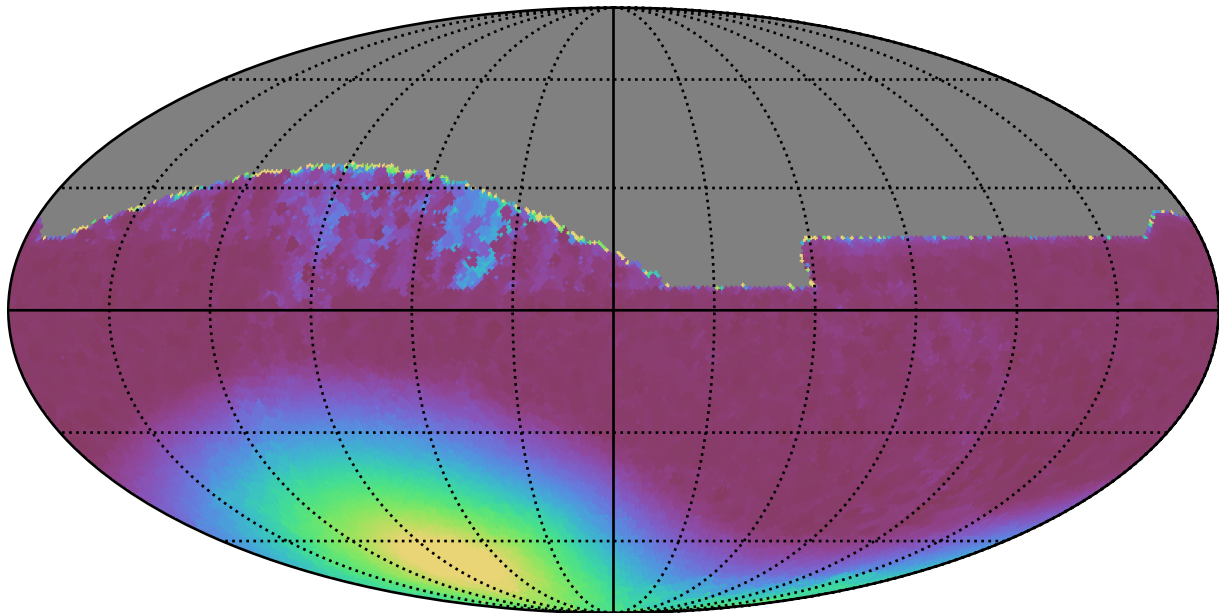
ddf_loaded_fl2_v3.4_10yrs All sky all bands: Min moonDistance
