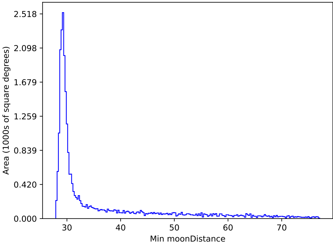
ddf_loaded_fl2_v3.4_10yrs All sky all bands: Min moonDistance
