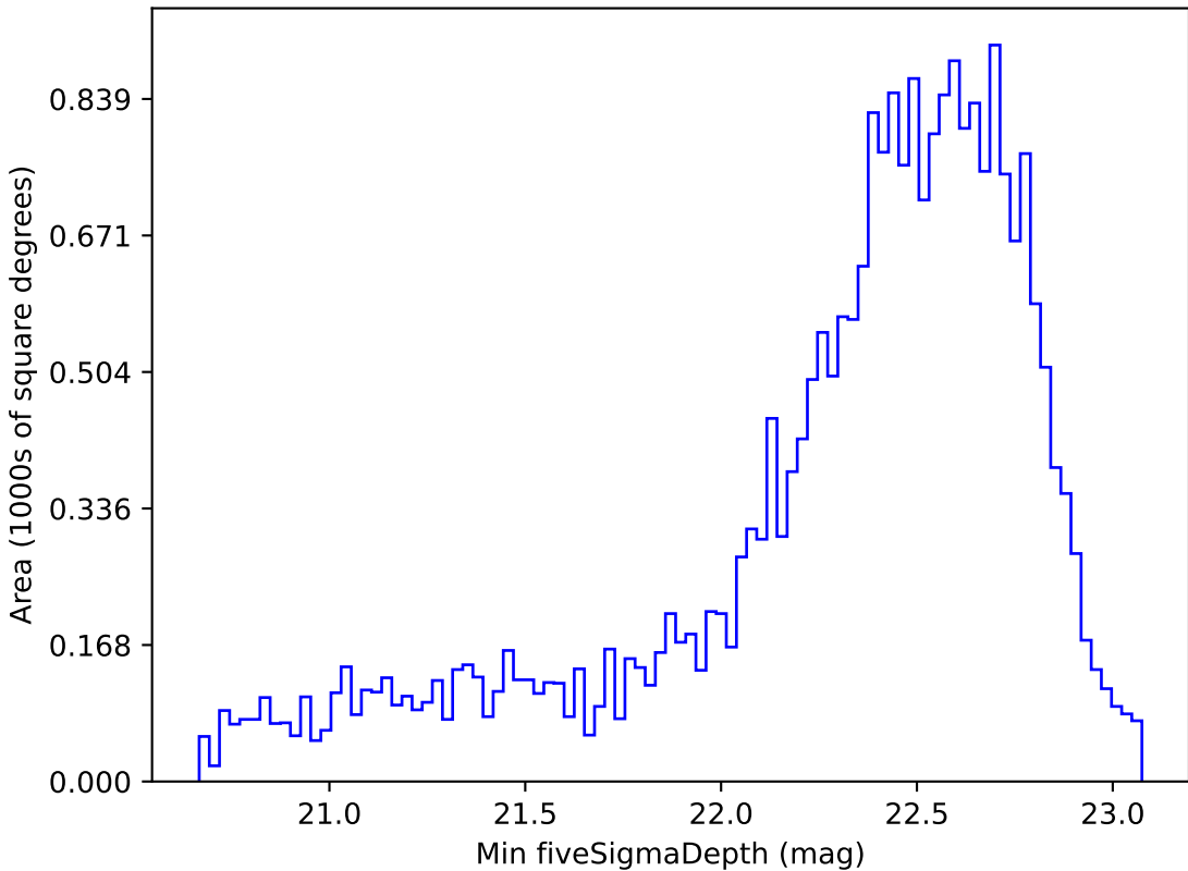
ddf_loaded_fl2_v3.4_10yrs Yr 1 z band: Min fiveSigmaDepth
