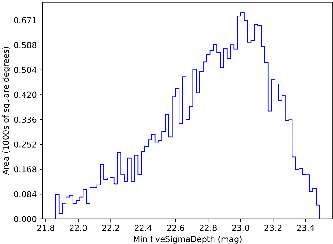
ddf_loaded_fl2_v3.4_10yrs Yr 1 u band: Min fiveSigmaDepth
