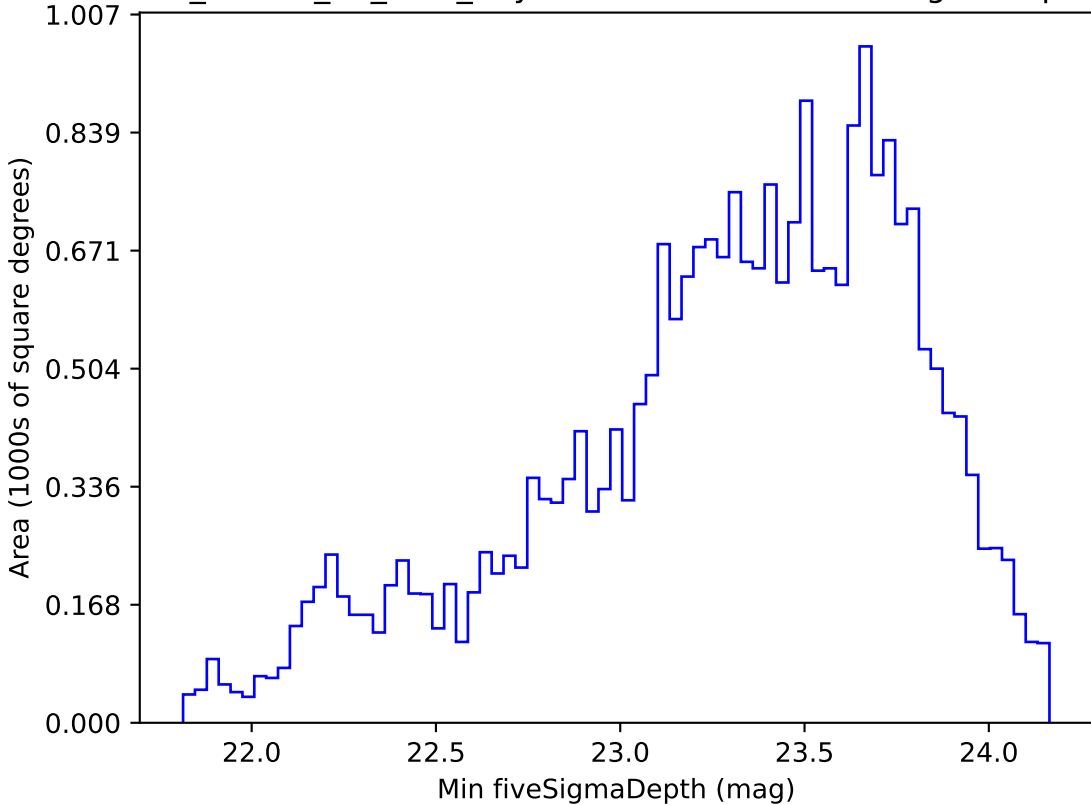
ddf_loaded_fl2_v3.4_10yrs Yr 1 r band: Min fiveSigmaDepth
