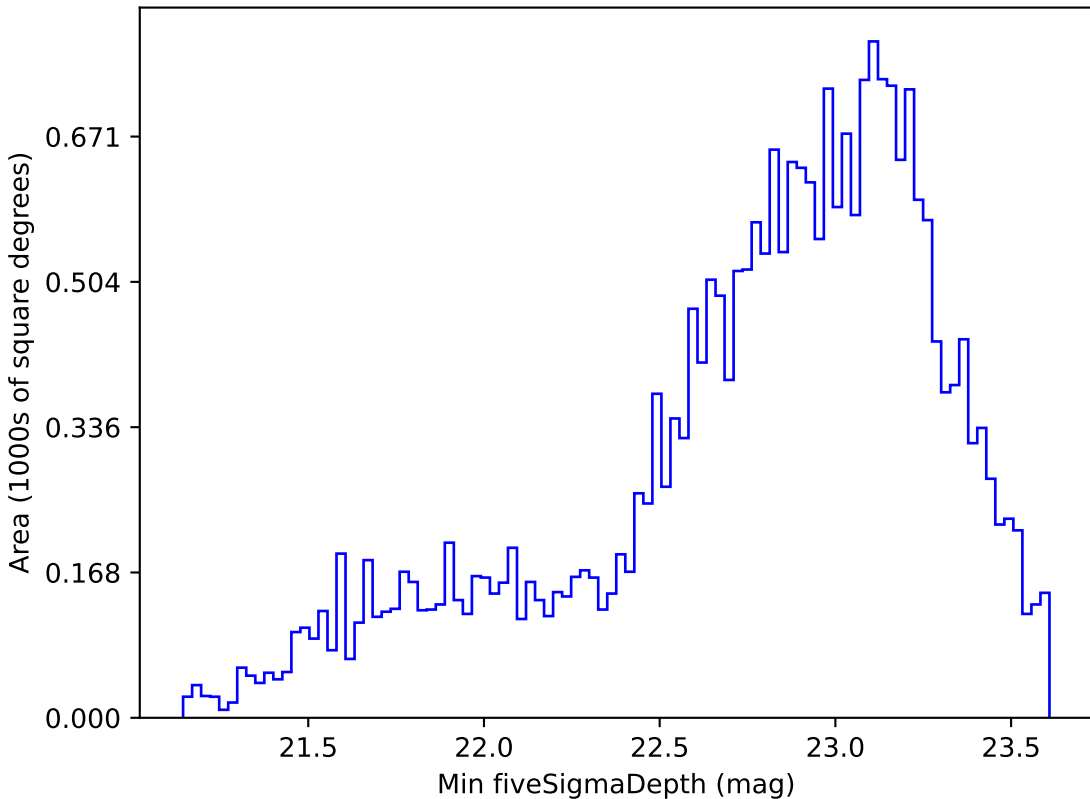
ddf_loaded_fl2_v3.4_10yrs Yr 1 i band: Min fiveSigmaDepth
