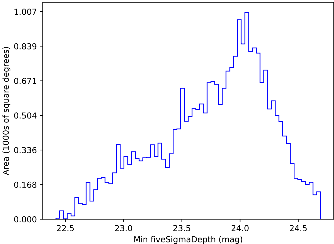
ddf_loaded_fl2_v3.4_10yrs Yr 1 g band: Min fiveSigmaDepth
