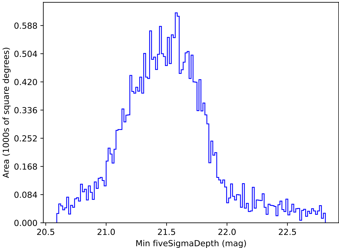
ddf_loaded_fl2_v3.4_10yrs Yr 1 all bands: Min fiveSigmaDepth
