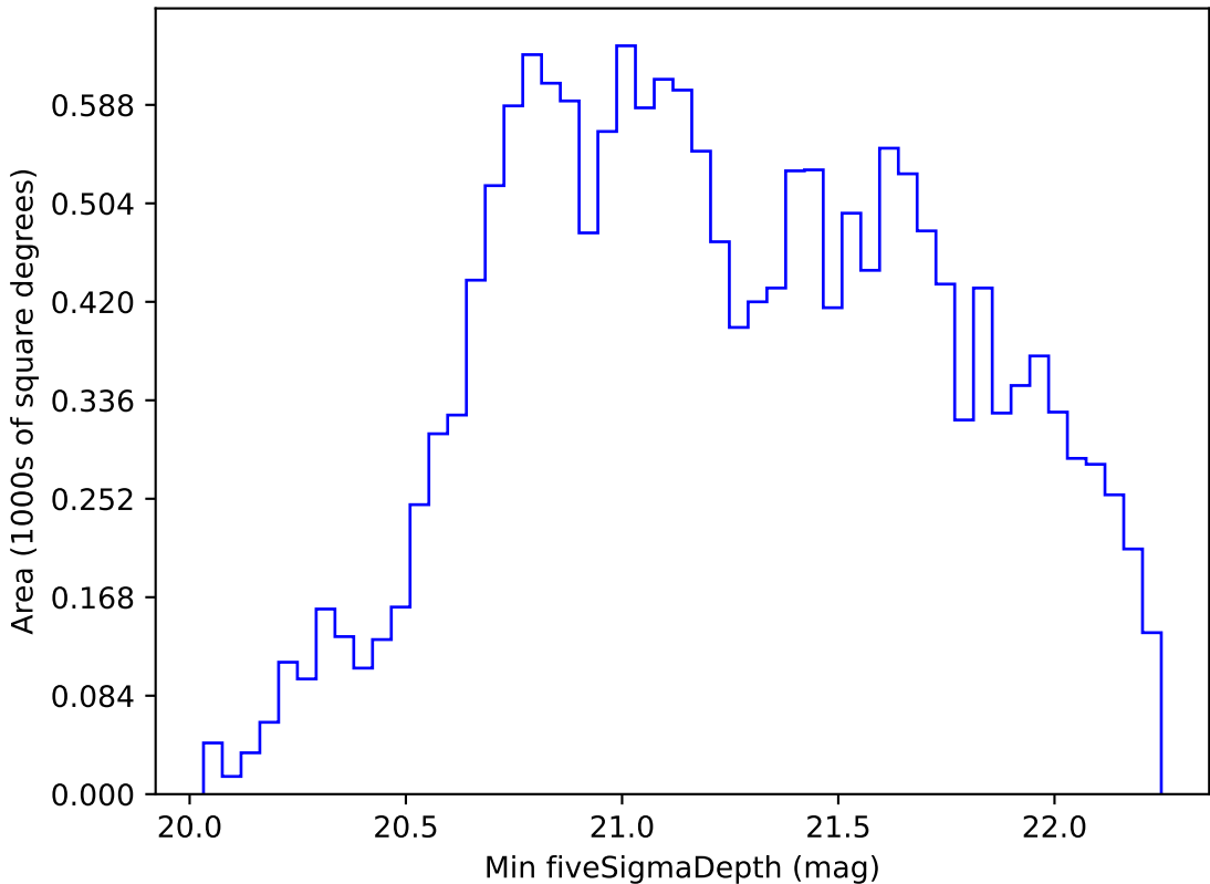
ddf_loaded_fl2_v3.4_10yrs WFD z band: Min fiveSigmaDepth
