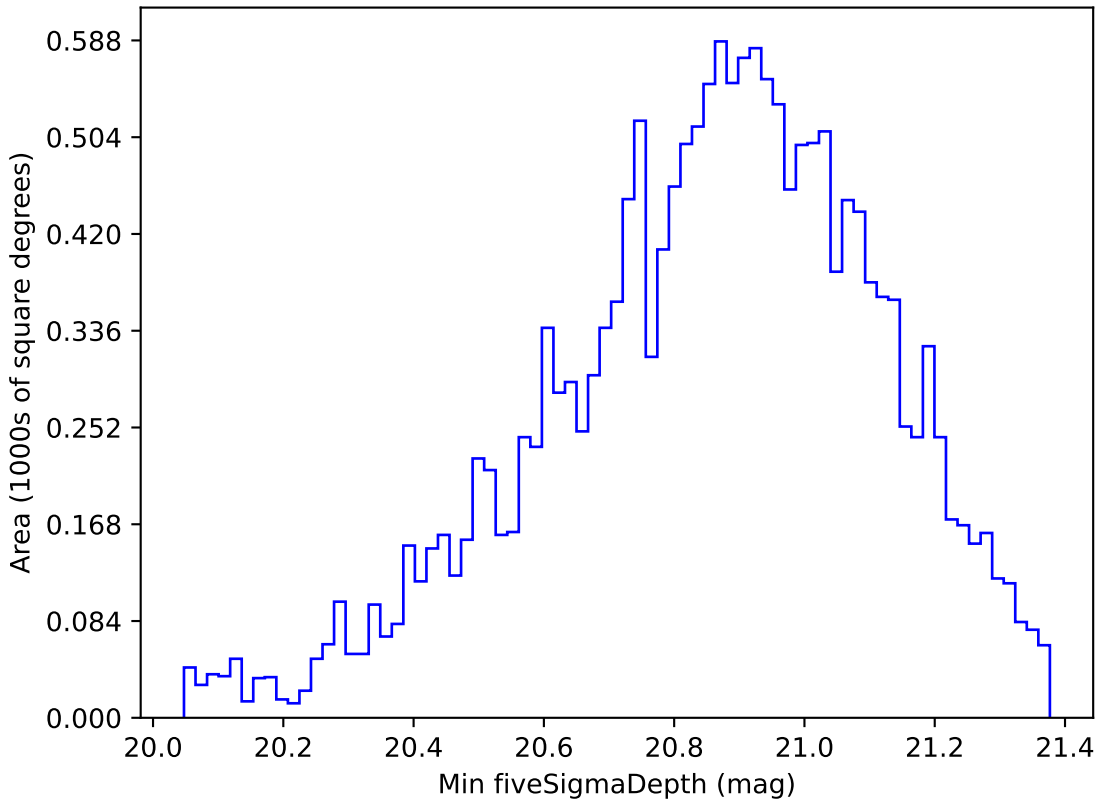
ddf_loaded_fl2_v3.4_10yrs WFD y band: Min fiveSigmaDepth
