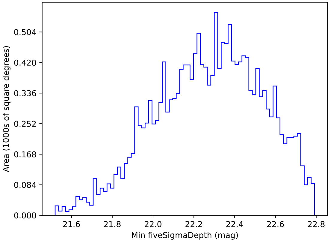
ddf_loaded_fl2_v3.4_10yrs WFD u band: Min fiveSigmaDepth
