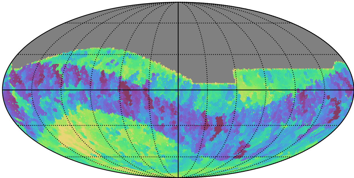
ddf_loaded_fl2_v3.4_10yrs All sky z band: Min fiveSigmaDepth
