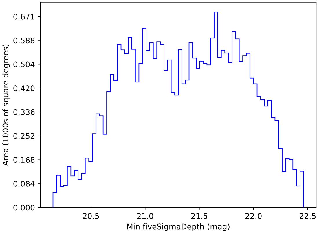
ddf_loaded_fl2_v3.4_10yrs All sky z band: Min fiveSigmaDepth
