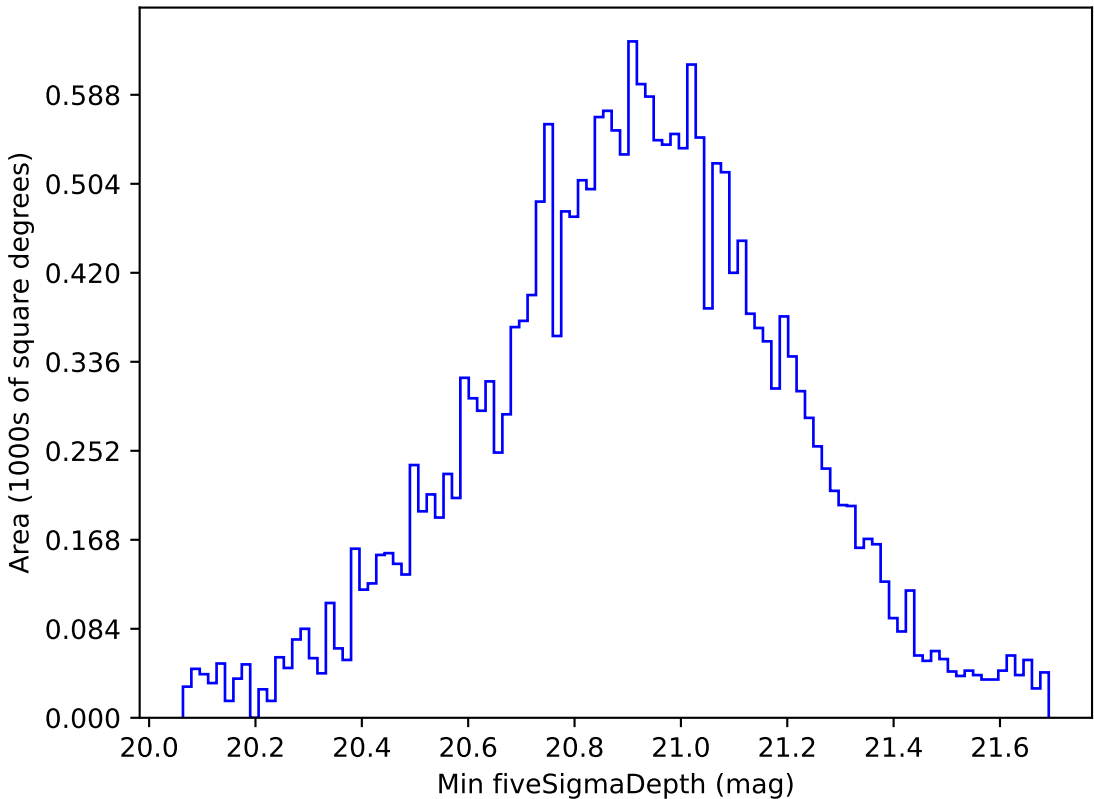
ddf_loaded_fl2_v3.4_10yrs All sky y band: Min fiveSigmaDepth
