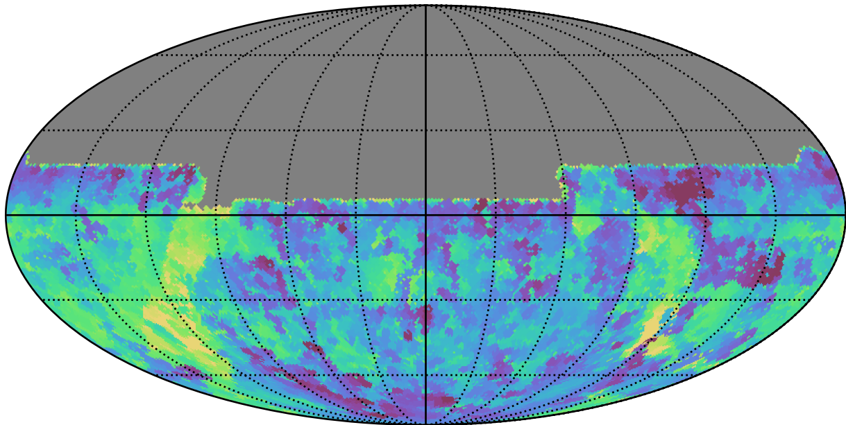
ddf_loaded_fl2_v3.4_10yrs All sky u band: Min fiveSigmaDepth
