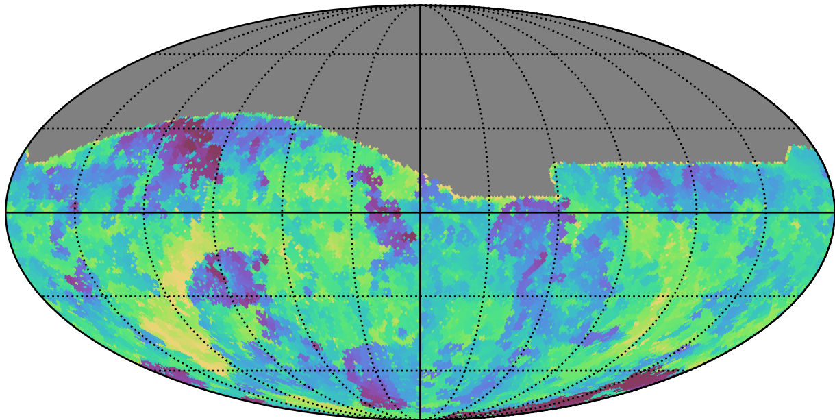
ddf_loaded_fl2_v3.4_10yrs All sky g band: Min fiveSigmaDepth
