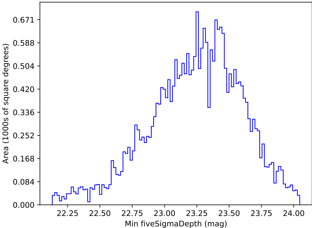
ddf_loaded_fl2_v3.4_10yrs All sky g band: Min fiveSigmaDepth
