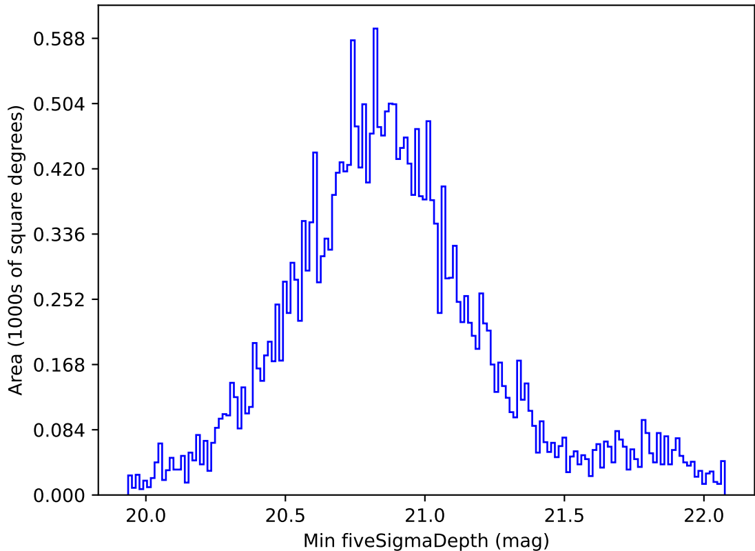
ddf_loaded_fl2_v3.4_10yrs All sky all bands: Min fiveSigmaDepth
