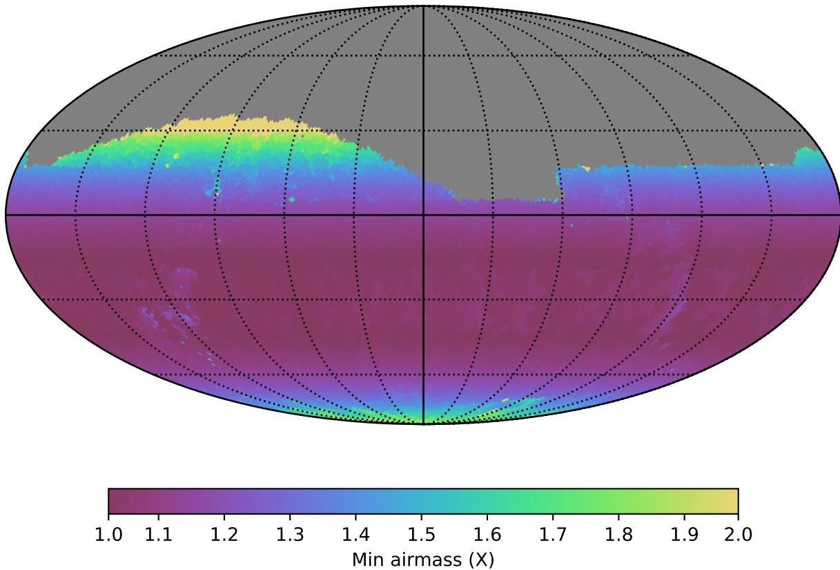
ddf_loaded_fl2_v3.4_10yrs Yr 1 z band: Min airmass
