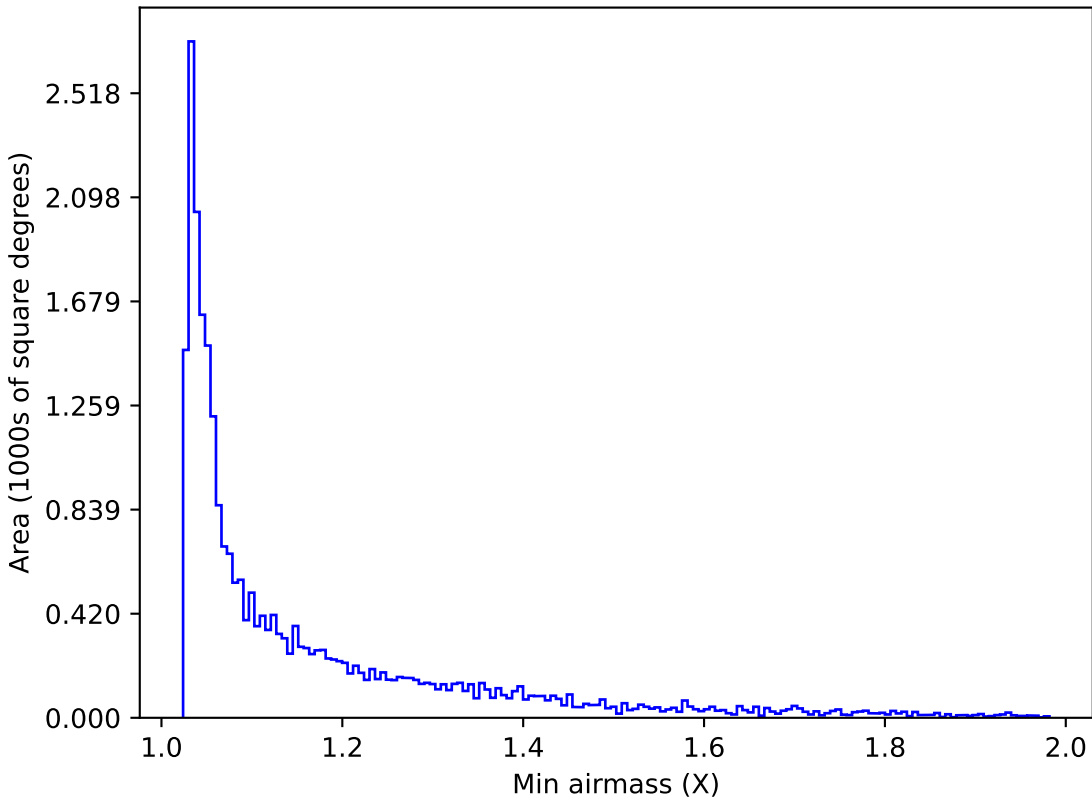
ddf_loaded_fl2_v3.4_10yrs Yr 1 z band: Min airmass
