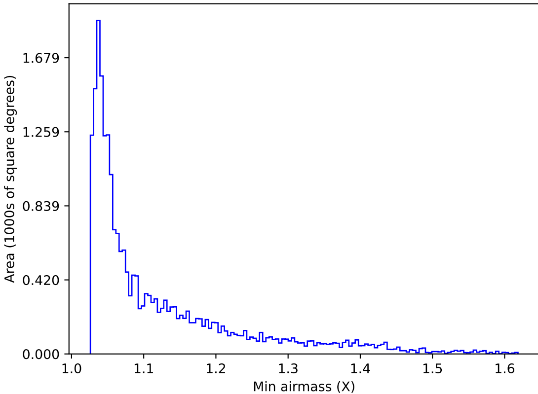
ddf_loaded_fl2_v3.4_10yrs Yr 1 y band: Min airmass
