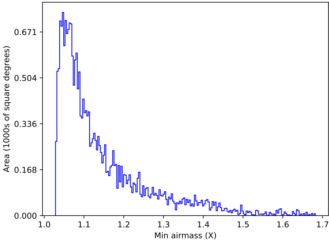
ddf_loaded_fl2_v3.4_10yrs Yr 1 u band: Min airmass
