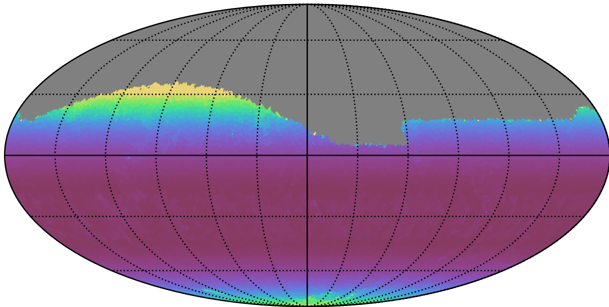
ddf_loaded_fl2_v3.4_10yrs Yr 1 r band: Min airmass
