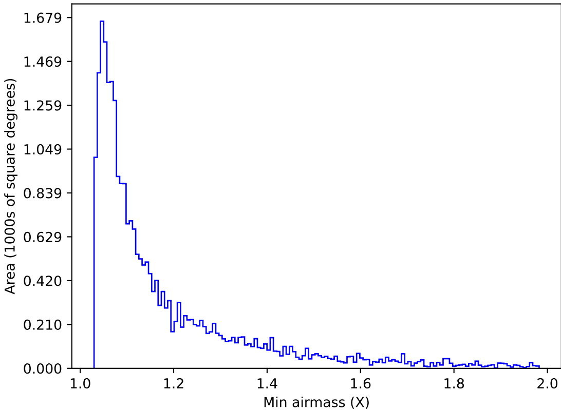
ddf_loaded_fl2_v3.4_10yrs Yr 1 g band: Min airmass
