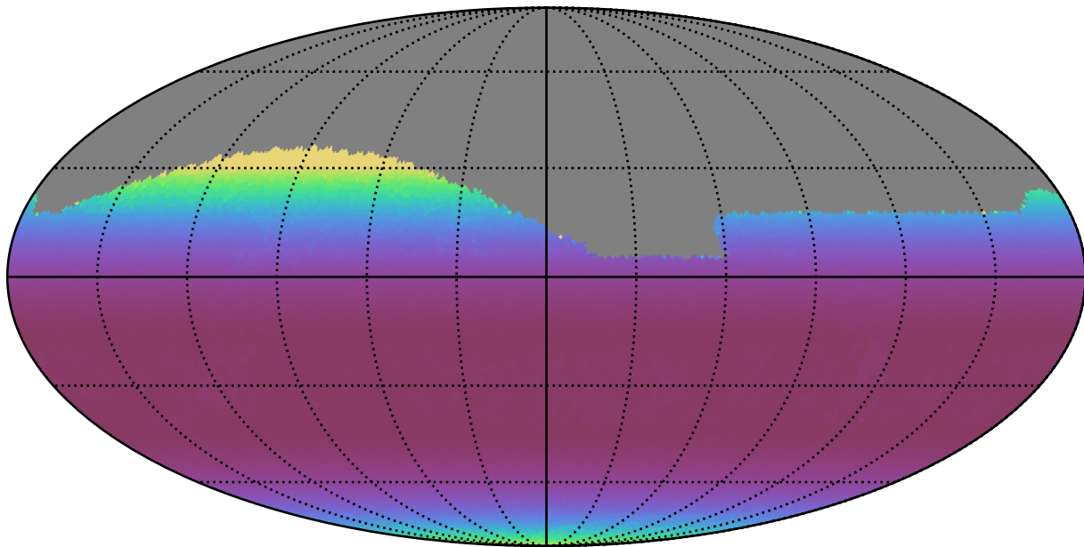
ddf_loaded_fl2_v3.4_10yrs Yr 1 all bands: Min airmass
