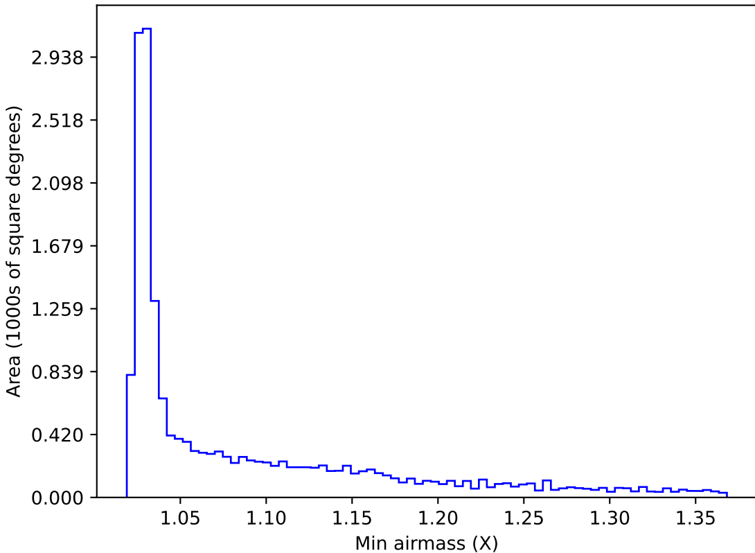
ddf_loaded_fl2_v3.4_10yrs WFD z band: Min airmass
