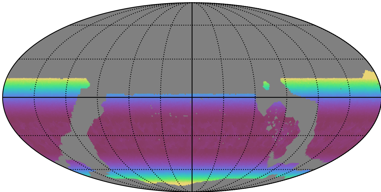
ddf_loaded_fl2_v3.4_10yrs WFD y band: Min airmass
