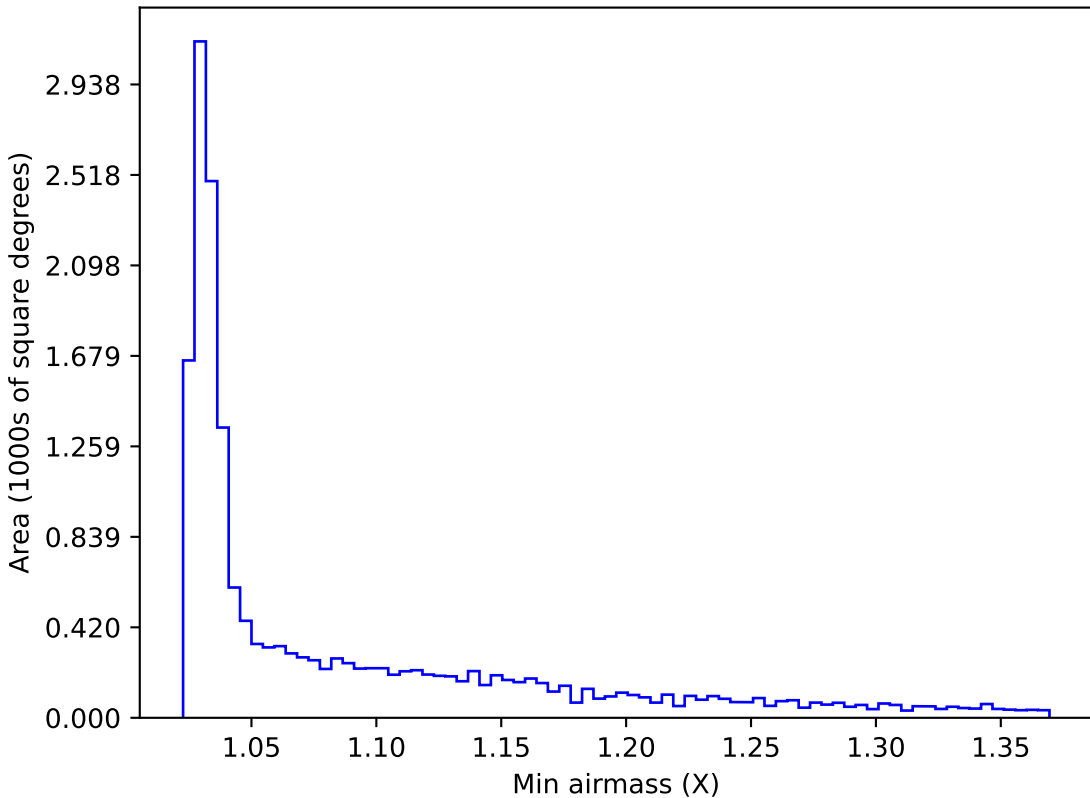
ddf_loaded_f12_v3.4_10yrs WFD y band: Min airmass
