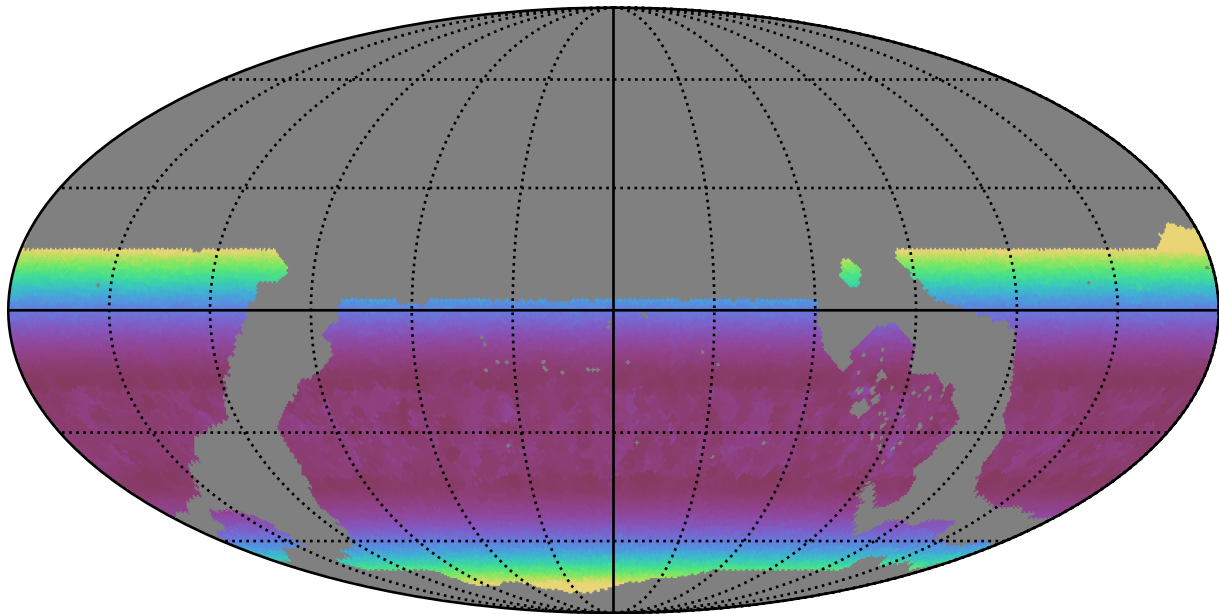
ddf_loaded_fl2_v3.4_10yrs WFD u band: Min airmass
