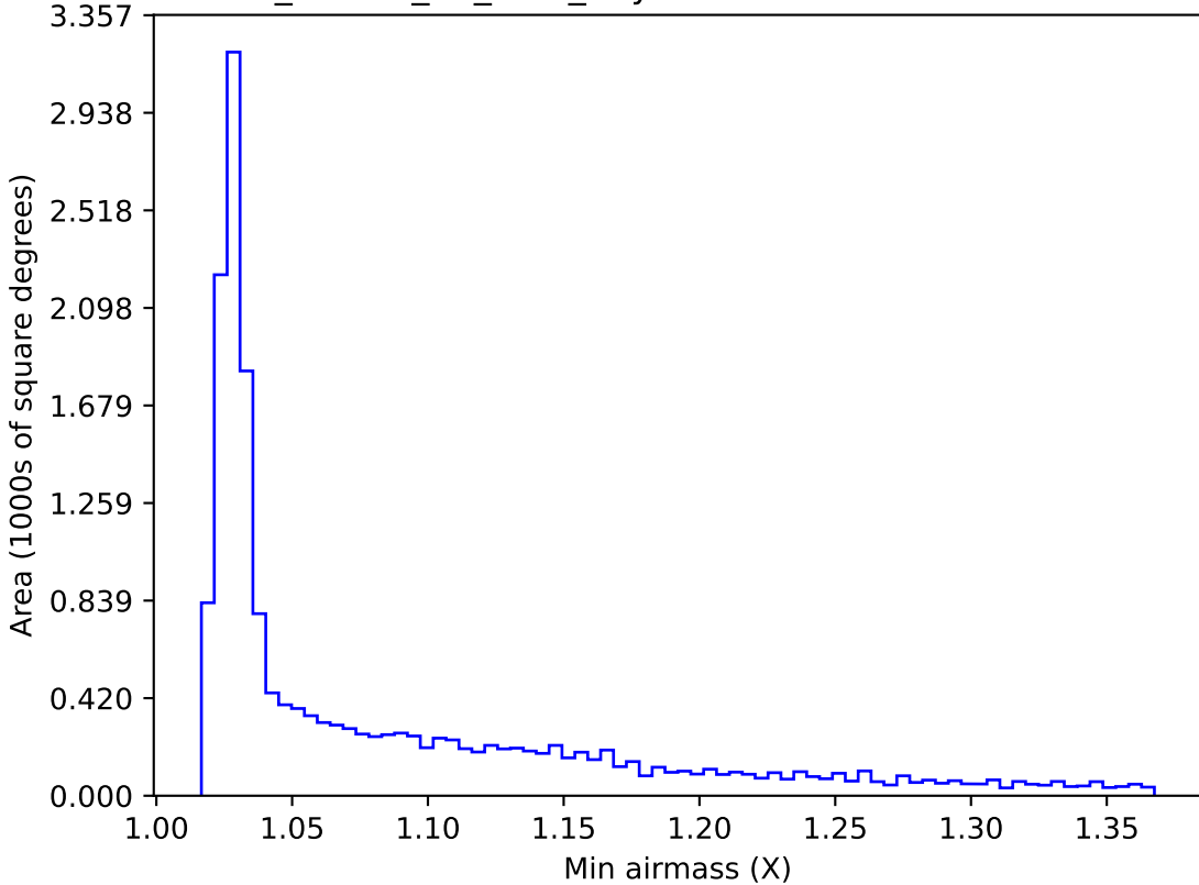
ddf_loaded_fl2_v3.4_10yrs WFD r band: Min airmass
