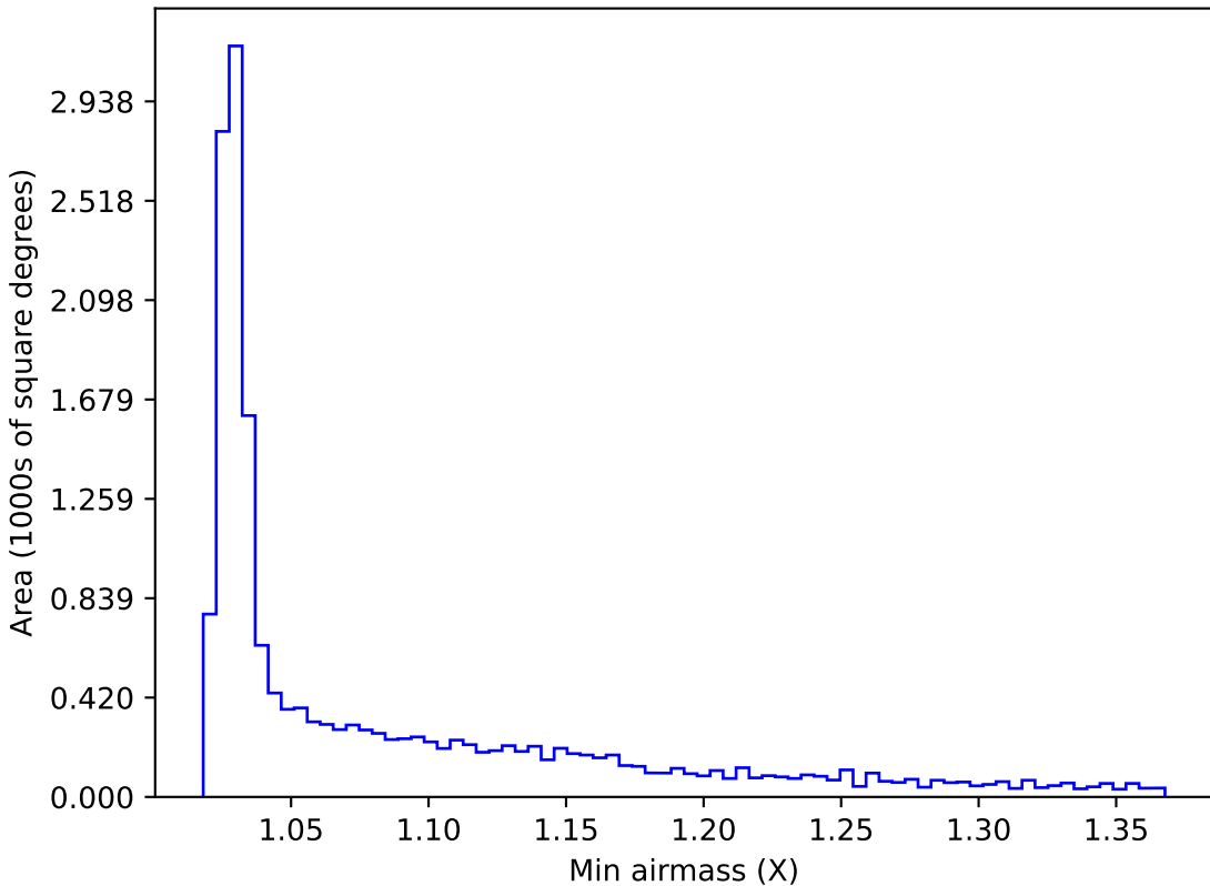
ddf_loaded_fl2_v3.4_10yrs WFD i band: Min airmass
