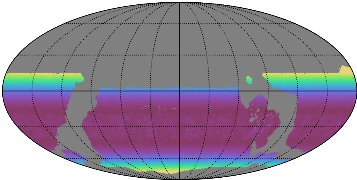
ddf_loaded_fl2_v3.4_10yrs WFD g band: Min airmass
