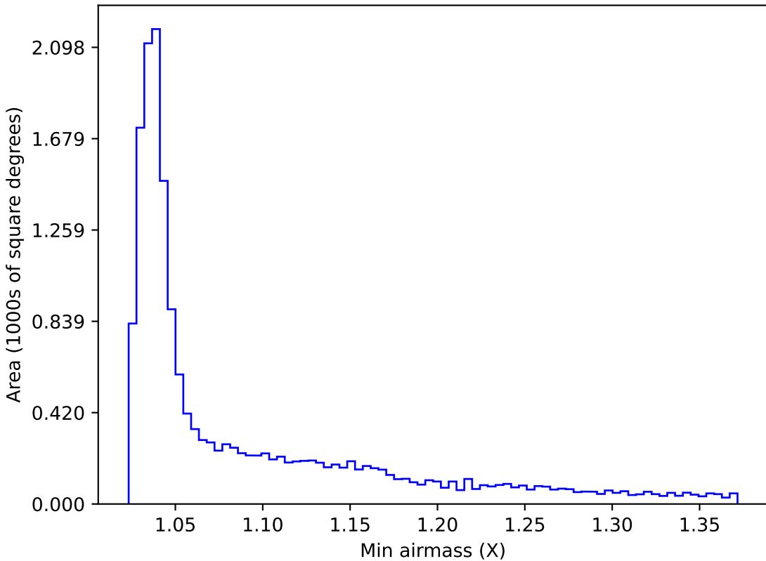
ddf_loaded_fl2_v3.4_10yrs WFD g band: Min airmass
