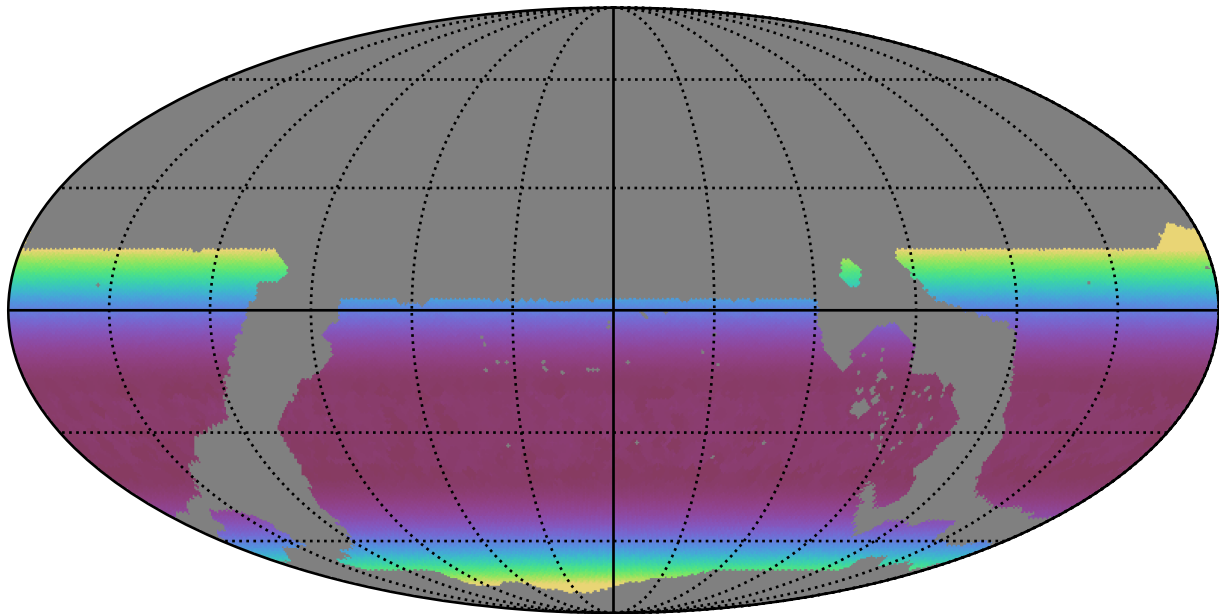
ddf_loaded_fl2_v3.4_10yrs WFD all bands: Min airmass
