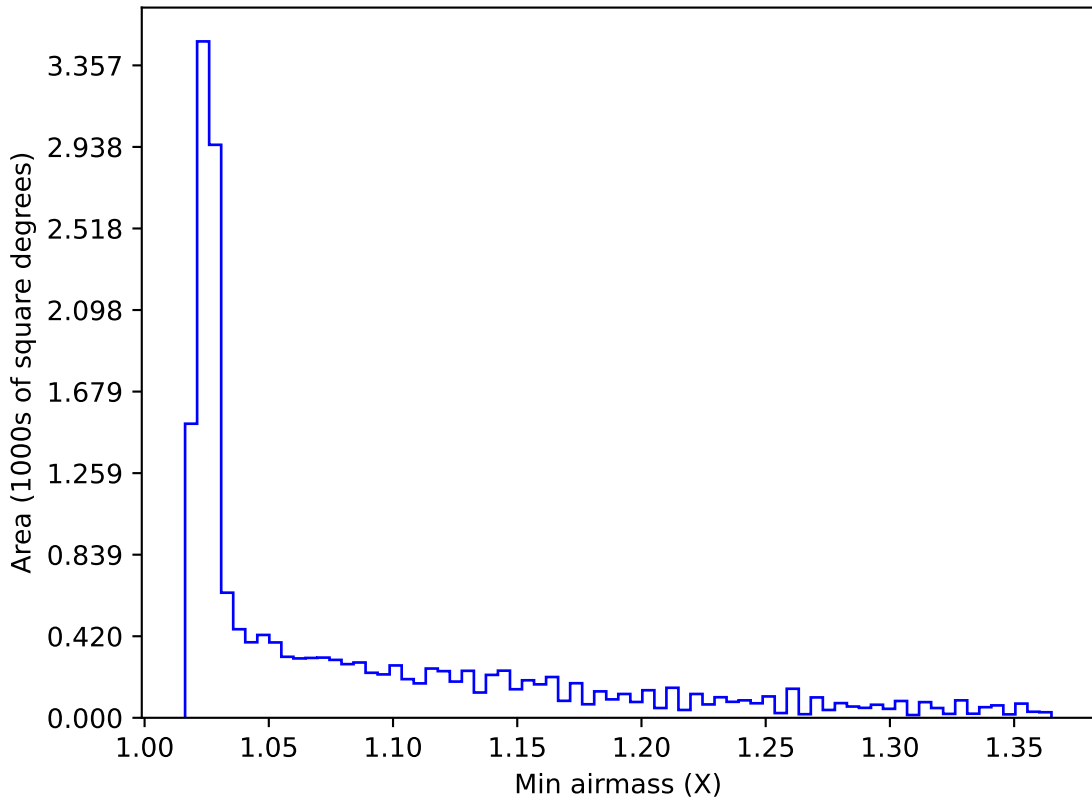
ddf_loaded_fl2_v3.4_10yrs WFD all bands: Min airmass
