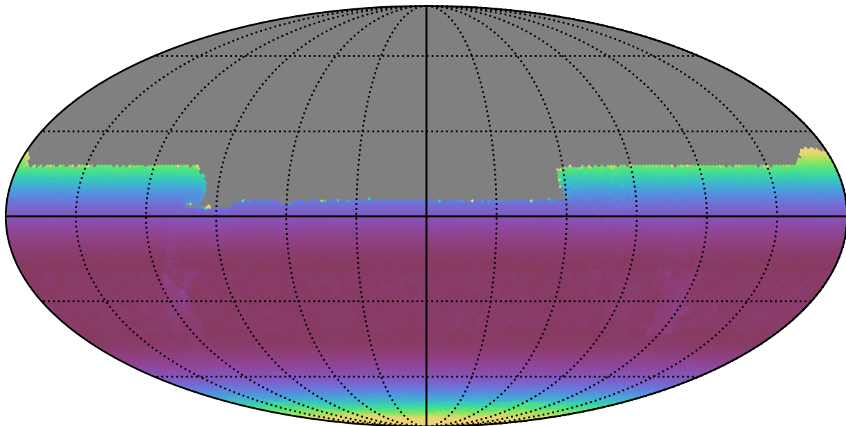
ddf_loaded_fl2_v3.4_10yrs All sky y band: Min airmass
