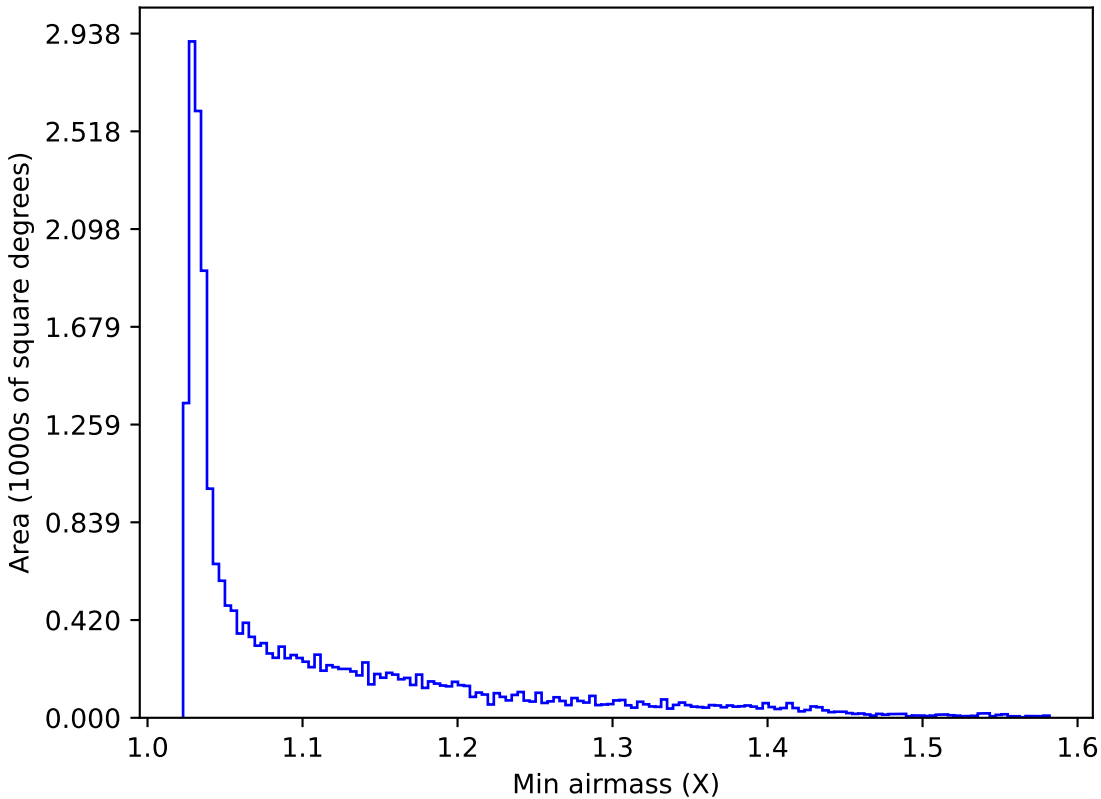
ddf_loaded_fl2_v3.4_10yrs All sky y band: Min airmass
